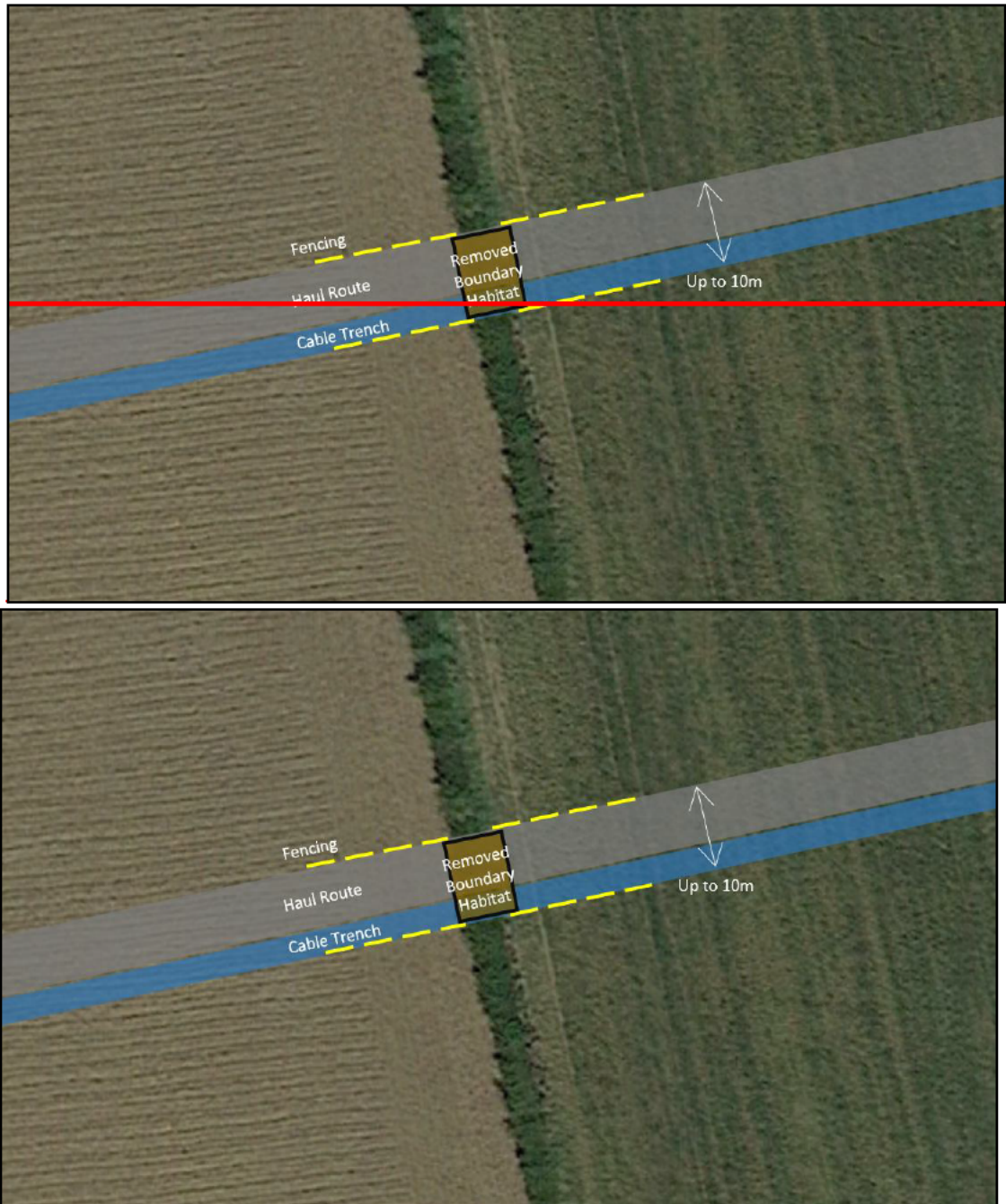
Figure 1. Indicative Layout of Protection Fencing at Boundary Habitat Crossings
